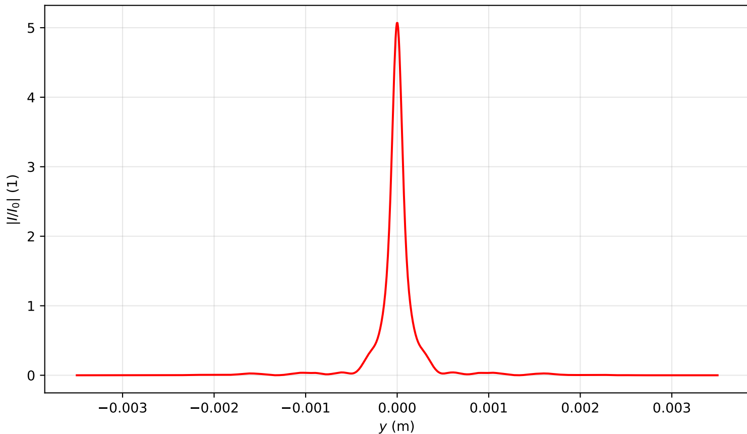
Intensity profile I(x=0, y, z=2.149)/I_0 , P_{in}=4.0P_{cr} , artificial time
